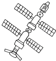
Space Station
